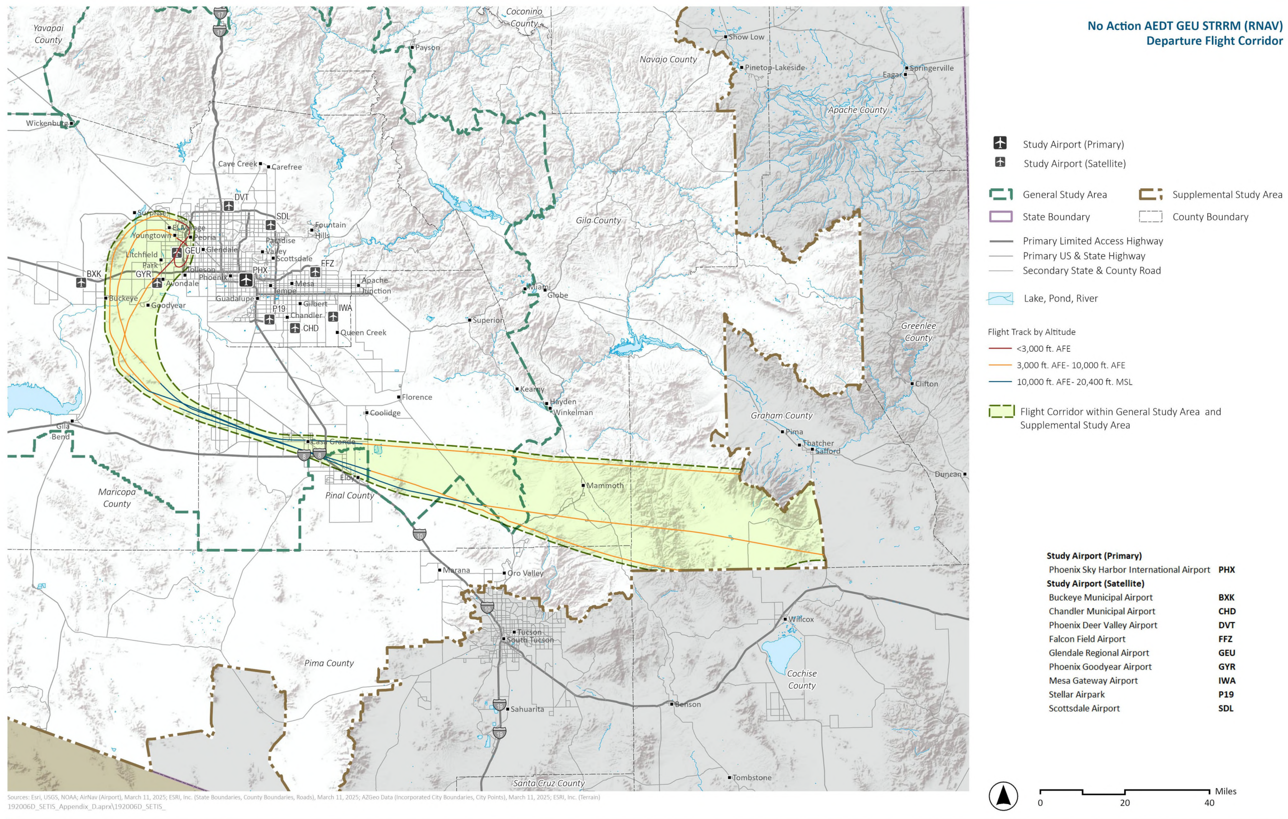
Exhibit H.6-14. No Action AEDT GEU STRRM (RNAV) Departure Flight Corridor
